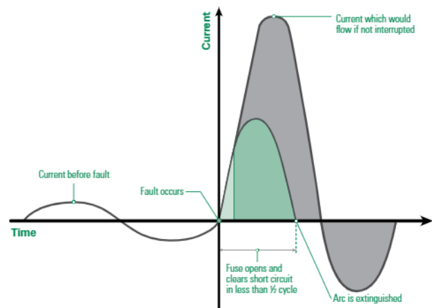
Figure 13 – Current-limiting Fuse
