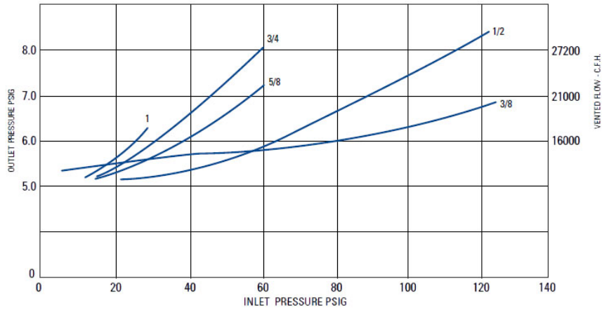
B38 IM RELIEF CURVES - BLOCKED PER ORIFICE 5 PSIG SET POINT
