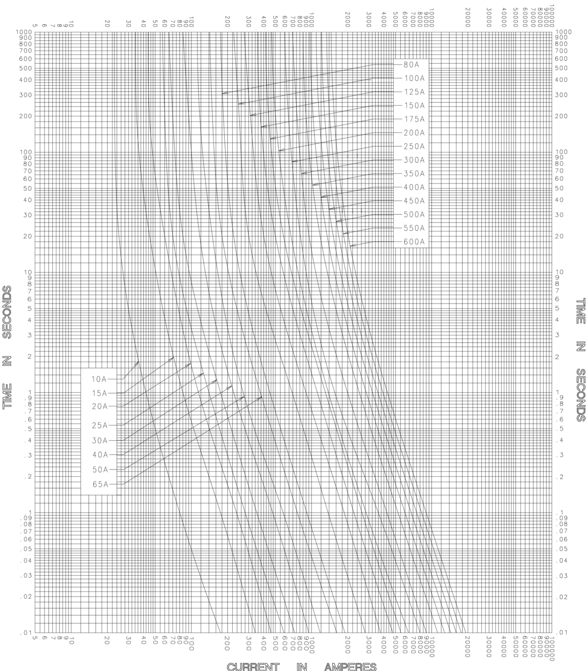
CLEARING TIME CURRENT CHARACTERISTIC CURVES
