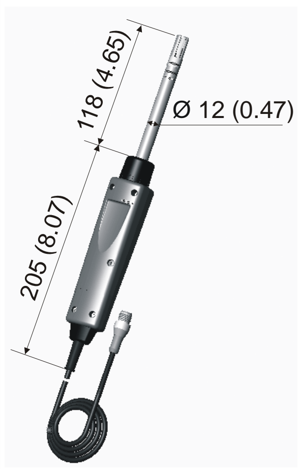
HMP75 Probe
