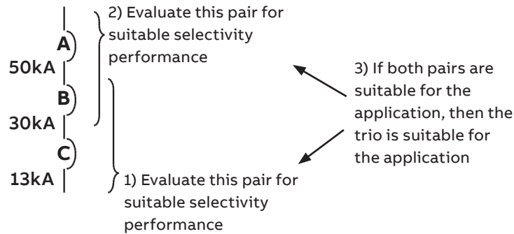
Figure 2: Multiple circuit breaker selectivity
