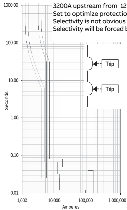
Figures 6 & 7: Selectivity with respect to current over time
