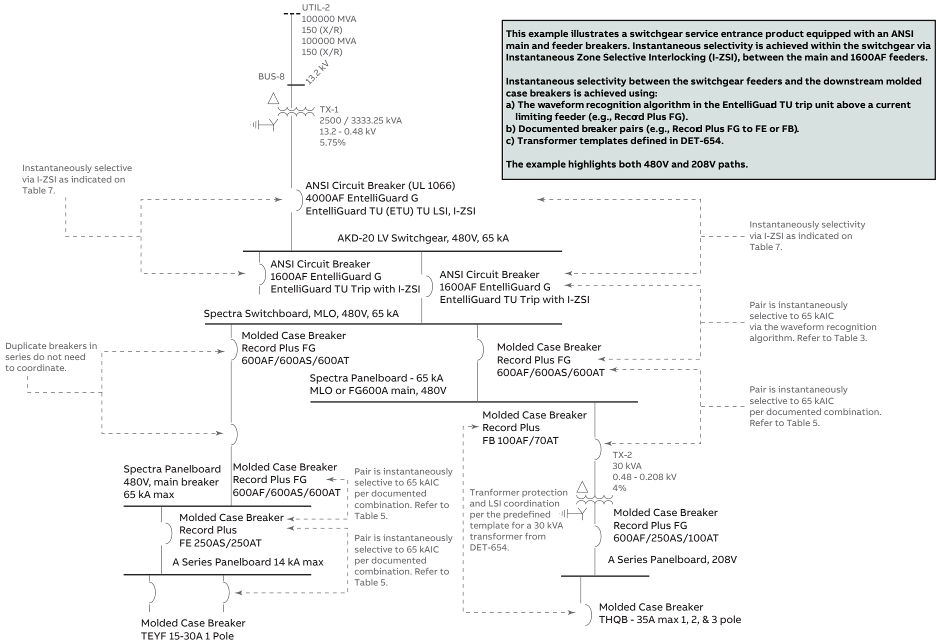
Figure 5: Selectivity using ArcWatch I-ZSI and WFR tested breaker pairs with switchgear service entrance, 480V and 208V paths
